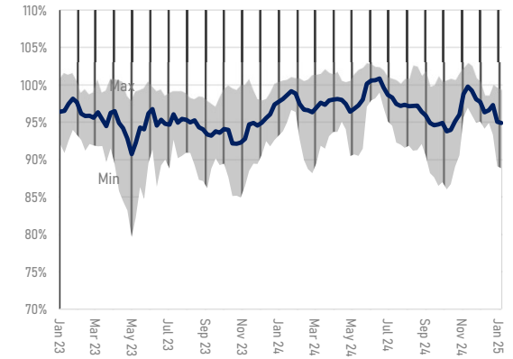
THE Alliance: FE-NEUR Head Haul Utilization
